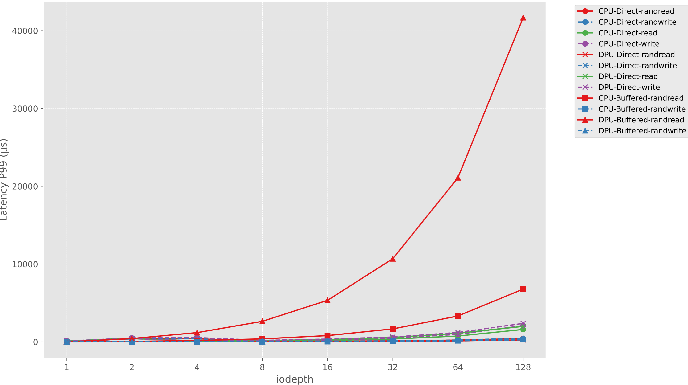
Latency P99 vs iodepth (CPU vs DPU, Direct vs Buffered)
